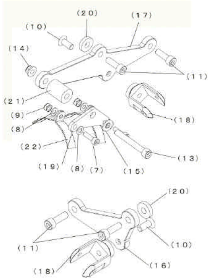
Drawing 1: how to attach a silencer stay
