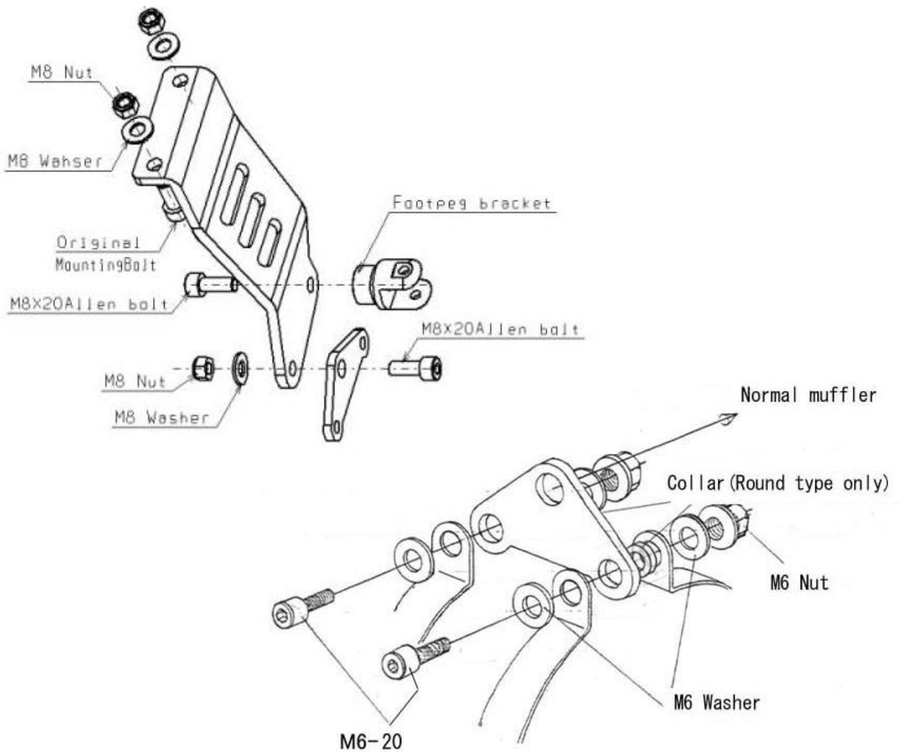
Fig. 3 How to attach the silencer band stay
